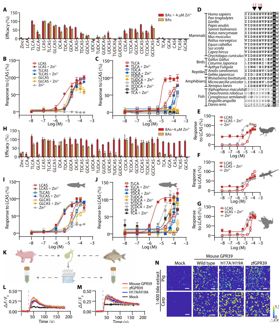
Fig. 4. Evolution of Zn^{2+} responsiveness after BA responsiveness in GPR39. (A) Efficacy of BAs in Zn^{2+} insensitive GPR39 mutant H17A/H19A activation in the presence or absence of 4 \mu M Zn^{2+} (means \pm s.e.m.; n = 3 or 4 in each group). All values were normalized to the efficacy of 200 \mu M LCAS. (B and C) Dose-response curves of H17A/H19A mutant form of GPR39 by BAs. Responses were normalized to 200 \mu M LCAS. (D) Multiple sequence alignment of GPR39 receptors from different species. The ClustalW program was used for sequence alignment, and the figure was generated by ESRIpt3. For each sequence, the accession number is shown in table S1. (E to G) Activation of G. gallus GPR39 (E), G. japonicus GPR39 (F), and X. laevis GPR39 (G) by LCAS and Zn^{2+} . (H) Efficacy of BA activation of the zfGPR39 in the presence or absence of 4 \mu M Zn^{2+} (means \pm s.e.m.; n = 3 or 4 in each group). All values were normalized to the efficacy of 200 \mu M LCAS. (I and J) Dose-response curves of the zfGPR39 by BAs. Responses were normalized to 200 \mu M LCAS. (K) Raw bile samples from pigs and carp were subjected to extraction using a C18 solid-phase cartridge. The crude extracts were employed to assess the responses of GPR39 to both pig and fish bile. (L and M) FLIPR fluorescence curves of intracellular Ca^{2+} changes induced by 1/400 diluted pig (L) and carp (M) bile extracts in HEK293T cells expressing mouse GPR39, zfGPR39, H17A/H19A mutant or mock-transfected cells. Dotted lines indicate the time points for the administration of agents. (N) Ca^{2+} imaging of GPR39-expressing HEK293T cells responding to 1/400 diluted pig and carp bile extracts. Scale bars, 100 \mu m .
