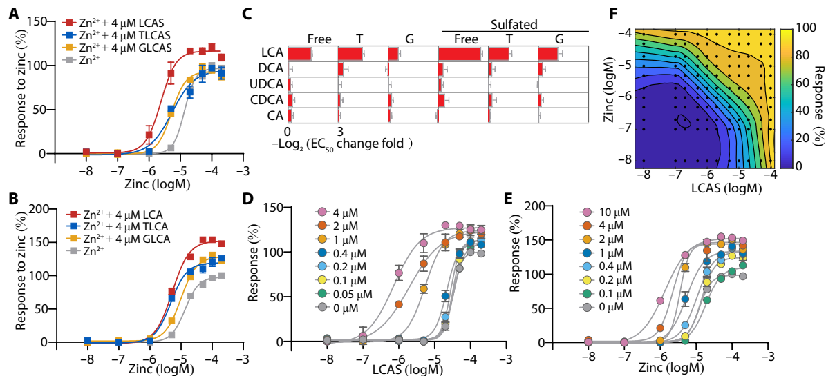
Fig. 3. LCA derivatives potentiate GPR39 activation by \text{Zn}^{2+} . (A and B) The allosteric effect of LCA derivatives on GPR39 activation by \text{Zn}^{2+} . Responses were normalized to 200 \mu\text{M} \text{Zn}^{2+} . (C) The potentiation of 30 BAs on GPR39 activation by \text{Zn}^{2+} . The ratio of \text{EC}_{50} of \text{Zn}^{2+} in the presence of BAs to \text{EC}_{50} of \text{Zn}^{2+} in the absence of BAs was calculated, and the value was logarithmically (with a base of 2) transformed (means \pm s.e.m.; n = 3 or 4 in each group). Values are shown in fig. S8. (D) The dose curves of GPR39 activated by LCAS in the presence of indicated concentrations of \text{Zn}^{2+} . Responses were normalized to 200 \mu\text{M} LCAS. (E) The dose curves of GPR39 activated by \text{Zn}^{2+} in the presence of indicated concentrations of LCAS. Responses were normalized to 200 \mu\text{M} \text{Zn}^{2+} . (F) The LOWESS-fit response surface of GPR39 costimulated with combinations of LCAS and \text{Zn}^{2+} . Responses were normalized to the maximum response among all experimentally tested points (black dots).
