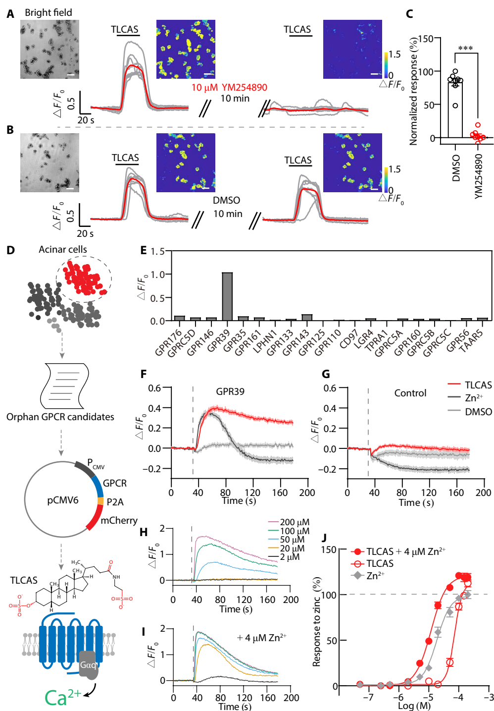
Fig. 1. Search for a TLCAS receptor. (A and B) \text{Ca}^{2+} imaging in isolated pancreatic acinar cells treated with \text{G}_{\alpha q} -inhibitor YM254890 (A) or vehicle dimethyl sulfoxide (DMSO) (B). Acinar cells were stimulated with two applications of 500 \mu\text{M} TLCAS. Before the second stimulation, the cells were incubated with 10 \mu\text{M} YM254890 (or DMSO) for 10 min. Red traces represent the average responses. Scale bars, 50 \mu\text{m} . (C) \text{G}_{\alpha q} -inhibitor YM254890 totally diminished the \text{Ca}^{2+} elevation induced by TLCAS in acinar cells. The values represent the responses of the second stimulation, which normalized to responses of the first stimulation. Two-tailed unpaired Student's t test was used ( ***P < 0.001 , n = 8 in each group). (D) A schematic diagram of our GPCR screening strategy. Orphan GPCRs highly expressed in pancreatic acinar cells were cloned and expressed in human embryonic kidney (HEK) 293T cells expressing \text{G}_{\alpha 15} -GCaMP6s, and possible activation of each receptor by TLCAS was measured by \text{Ca}^{2+} imaging. (E) Results of the intracellular \text{Ca}^{2+} changes mediated by candidate GPCRs in response to 200 \mu\text{M} TLCAS. (F and G) Real-time FLIPR fluorescence curves of intracellular \text{Ca}^{2+} changes induced by 200 \mu\text{M} TLCAS or 200 \mu\text{M} \text{Zn}^{2+} in GPR39-expressing cells (F) or the sham-transfected cells (G). The dotted line indicates the time points for the administration of agents or vehicles. (H) Concentration-dependent activation of GPR39 by TLCAS. Results from a stable HEK293T cell line expressing the GPR39 are shown here. (I) \text{Zn}^{2+} enhancement of GPR39 activation by TLCAS. Cells were incubated with 4 \mu\text{M} \text{Zn}^{2+} in the recording buffer for 5 min before the FLIPR assay, and the concentrations of TLCAS were similarly color-indicated as those in (H), except that 4 \mu\text{M} \text{Zn}^{2+} was included for all concentrations of TLCAS. (J) Dose curves of TLCAS and \text{Zn}^{2+} in GPR39 activation.
